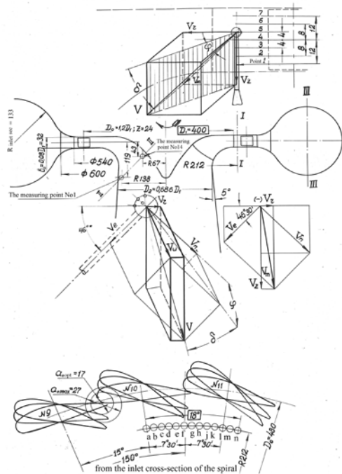
Fig. 3. The installation scheme of probes in measured sections of a model turbine
